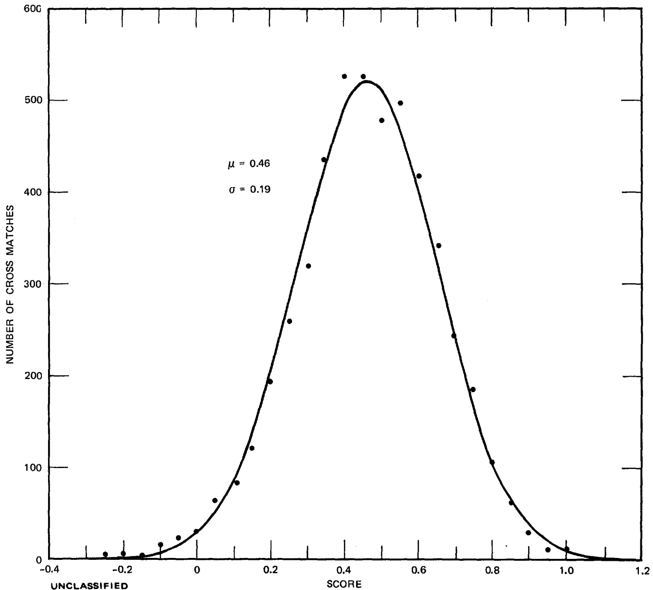
FIGURE 1 SCORE DISTRIBUTION FOR 4995 CROSS MATCHES
